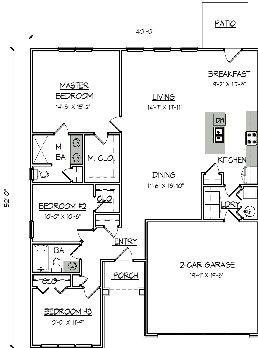
FLOOR PLAN
