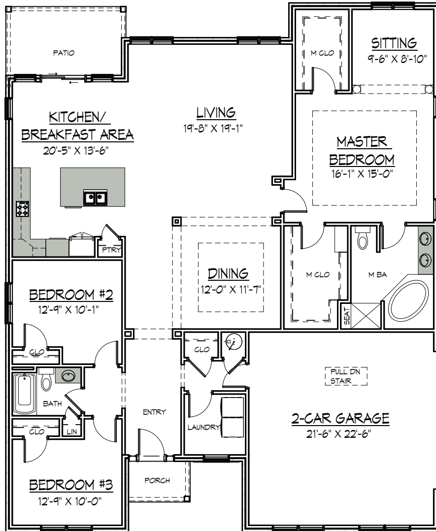
FLOOR PLAN
